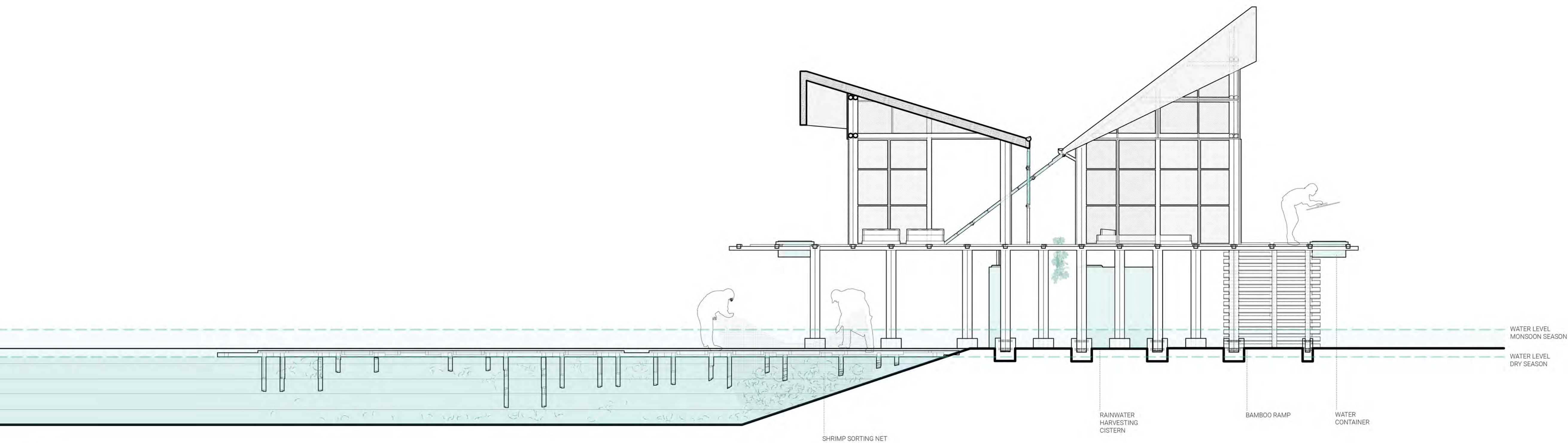
SECTION B
